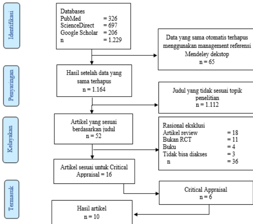
Gambar 1. PRISMA Flowchart
